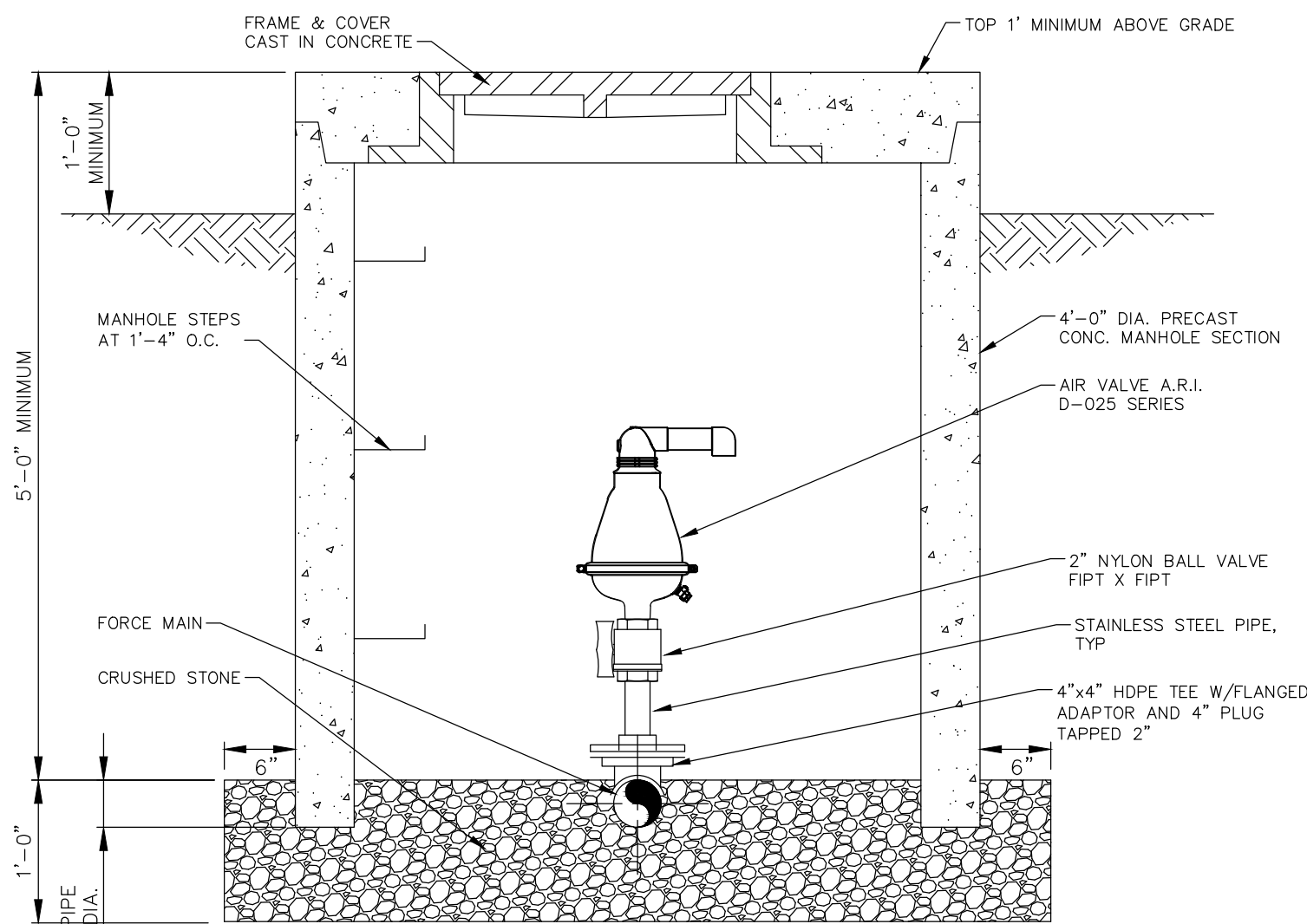
WASTEWATER COMBINATION AIR RELEASE VALVE & MANHOLE
