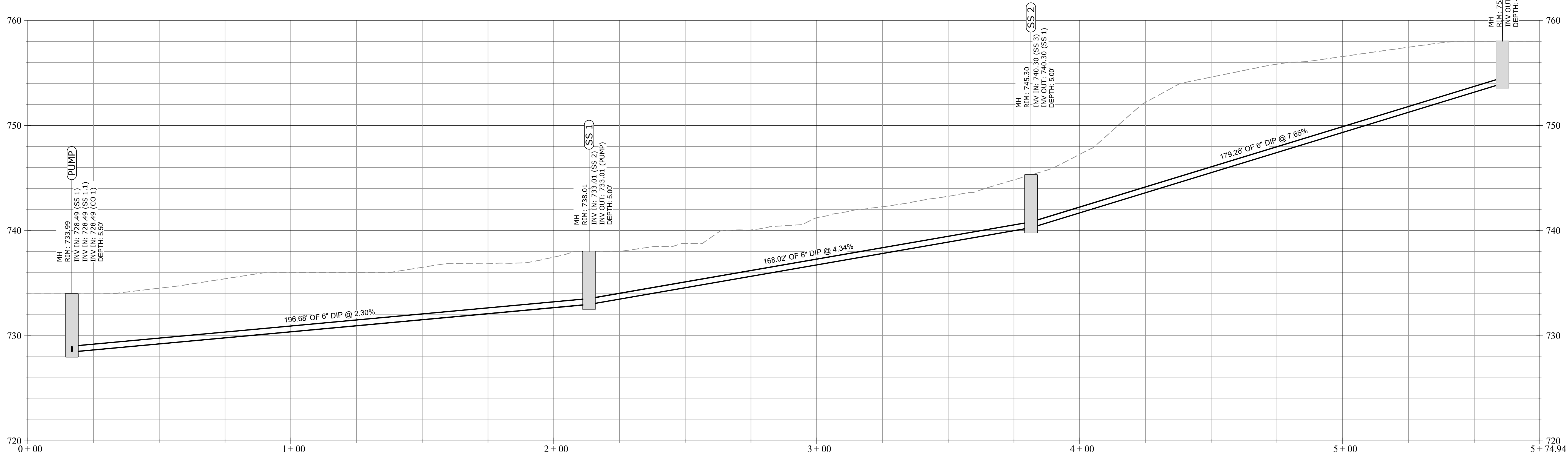
① PUMP - SS 3 SANITARY SEWER PROFILE H: 1" = 20' V: 1" = 4' 0 10' 20' 40' 0 2' 4' 8'
