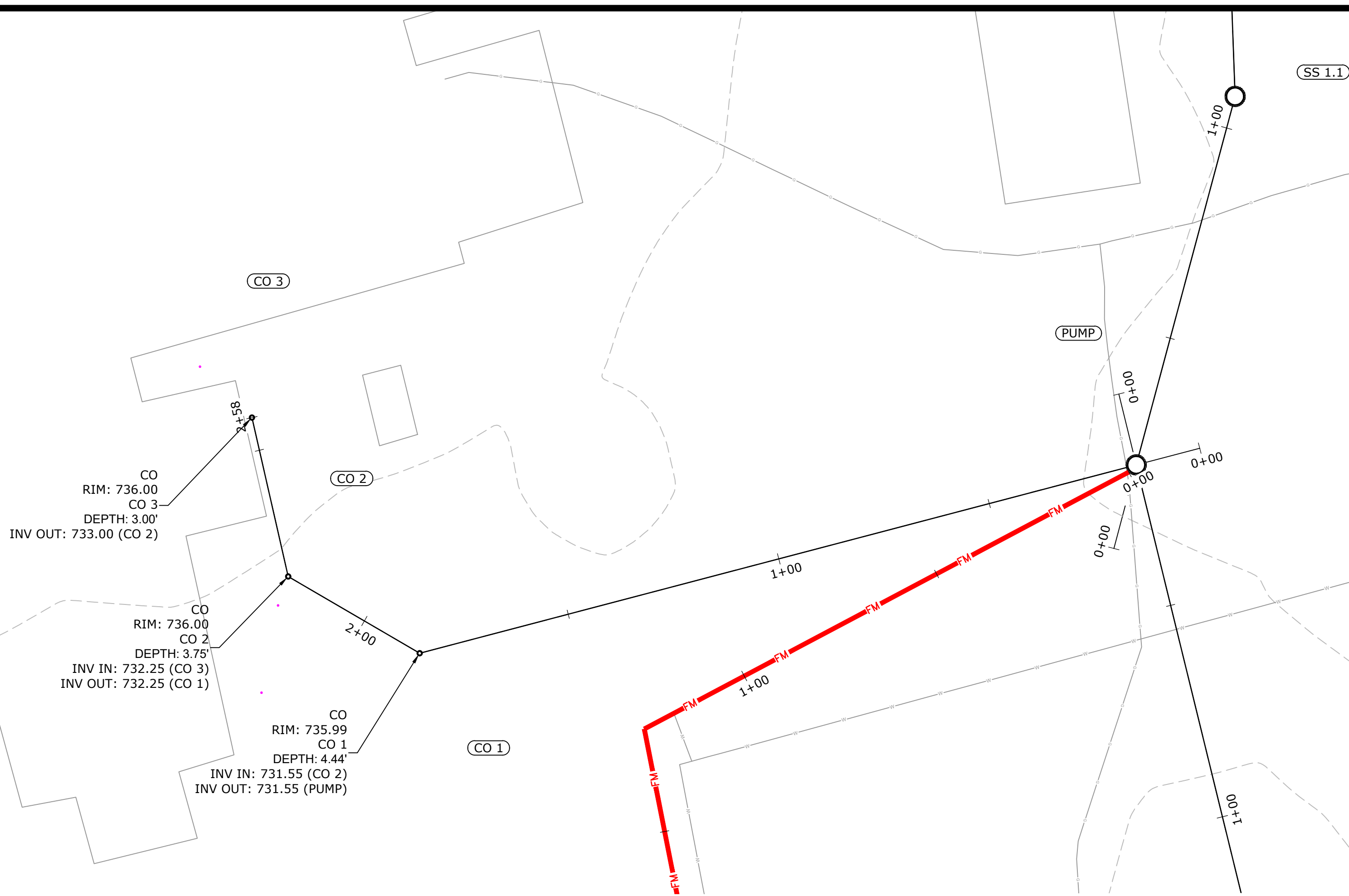
① PUMP TO CLEAN OUT 3 - PLAN VIEW
