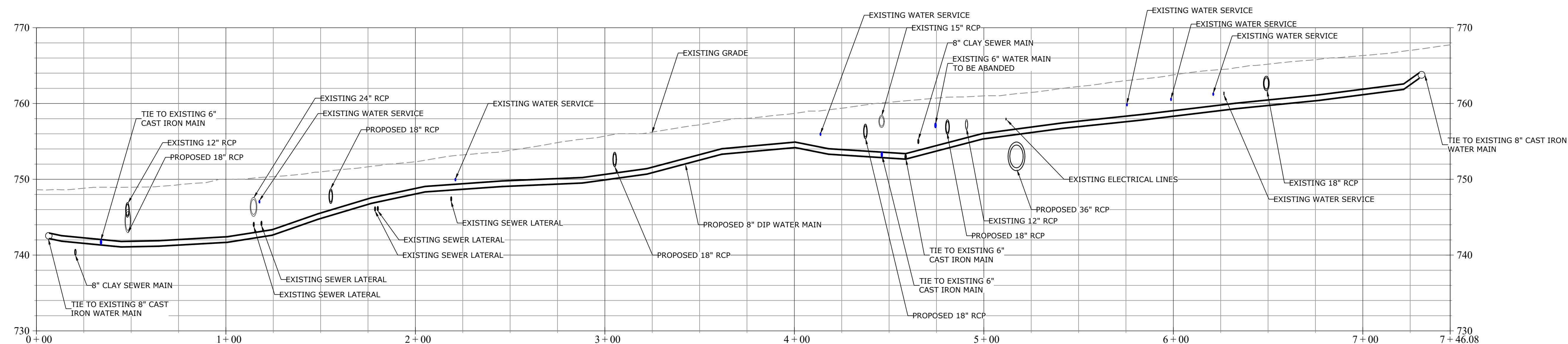
1 PENTZ ST - PROFILE H: 1" = 30' V: 1" = 4'
