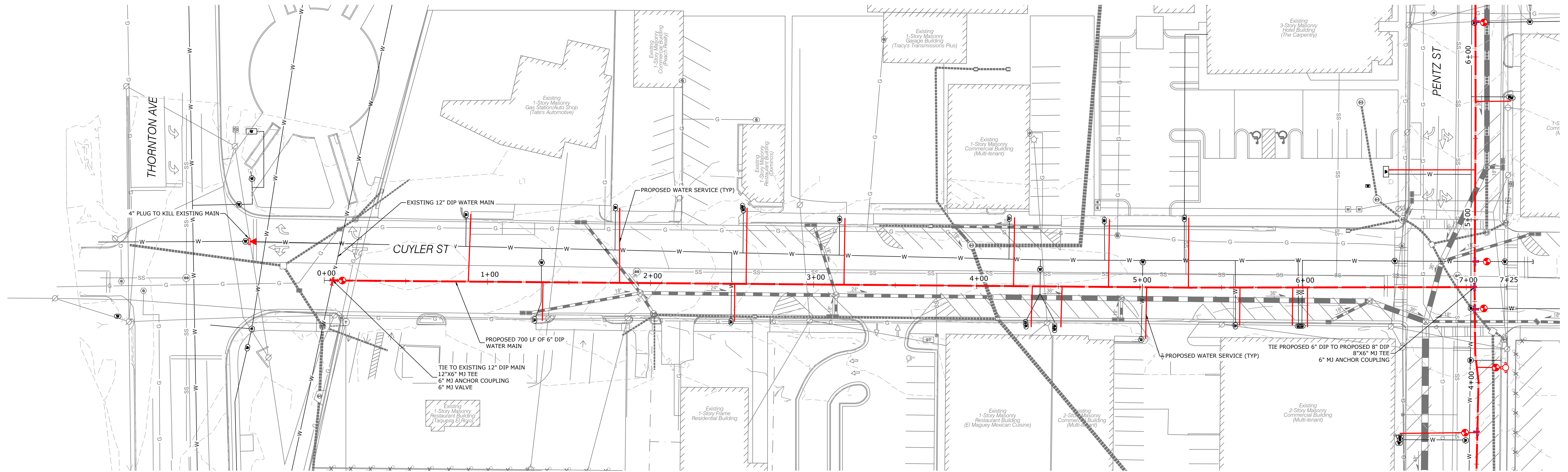
① CUYLER ST - PLAN VIEW 1" = 30' 0 15' 30' 60'
