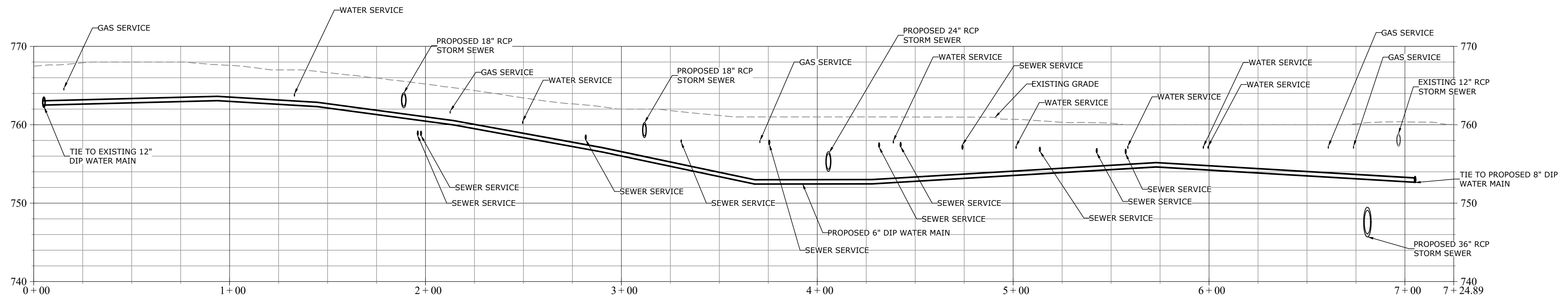
① CUYLER ST - PROFILE H: 1" = 30' 0 15' 30' 60' V: 1" = 4' 0 2' 4' 8'
