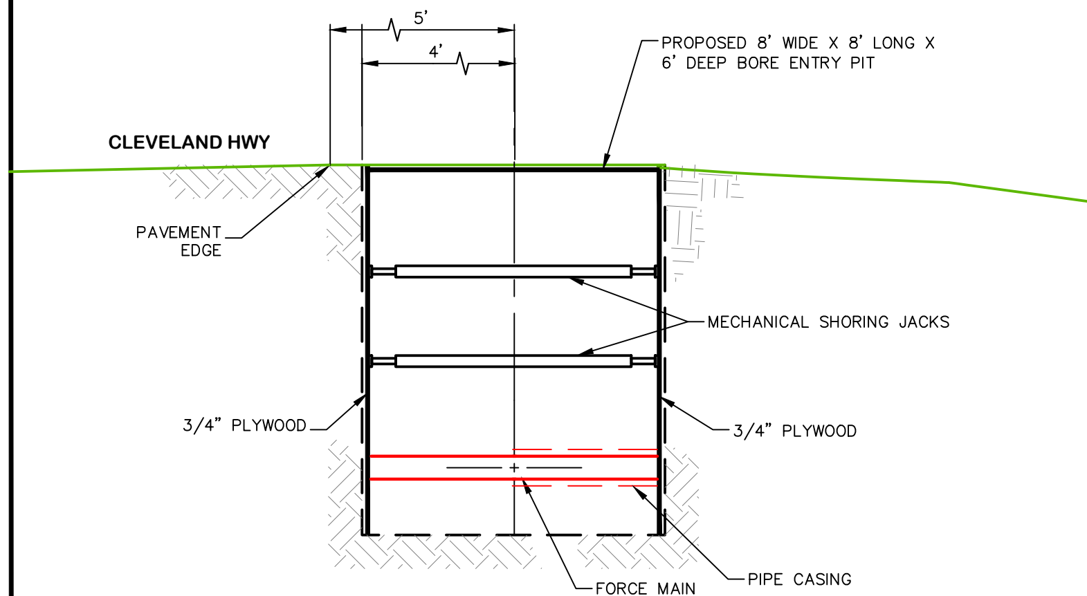
PROPOSED BULKHEAD TO PROTECT ROAD BED AND PERSONNEL N.T.S.
